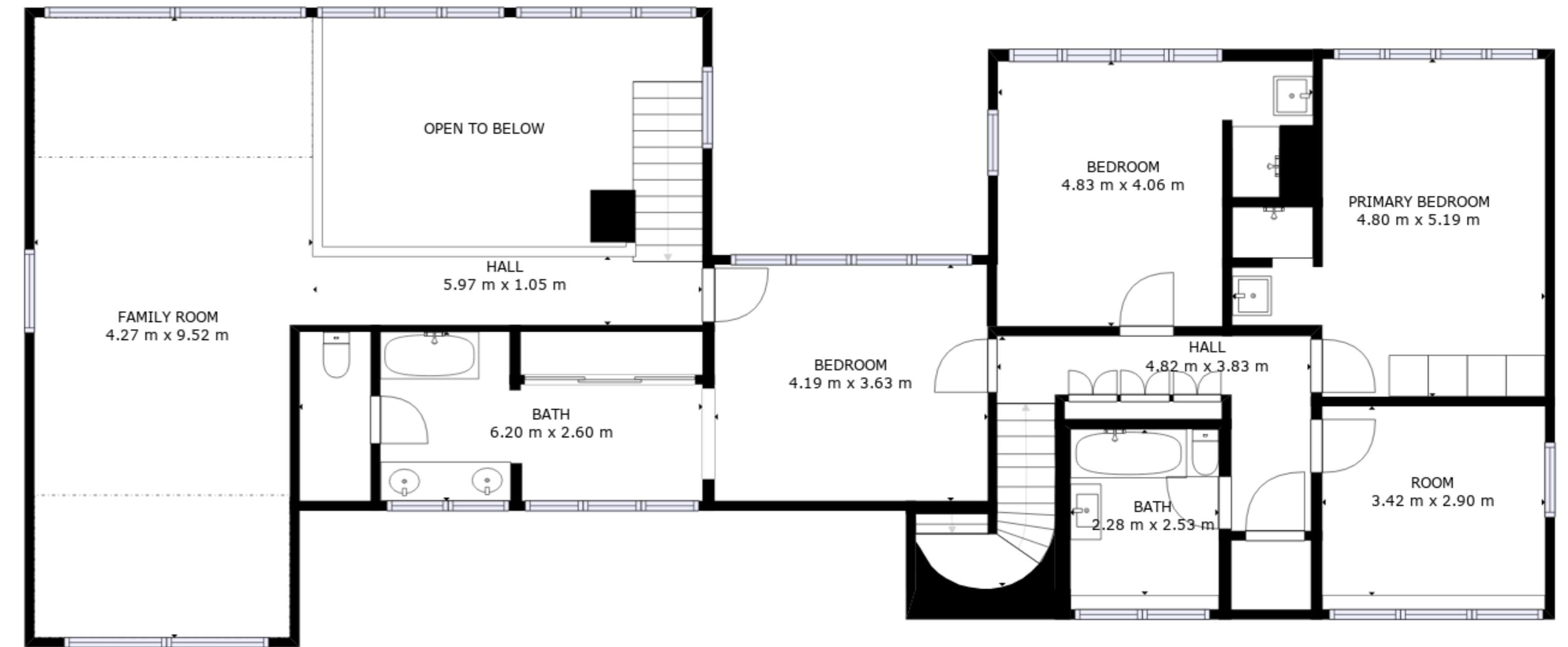
FLOOR 3
